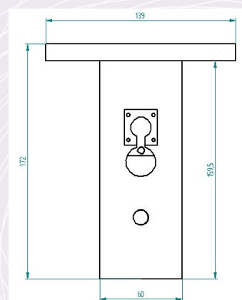
Main dimensions of the MS1:
